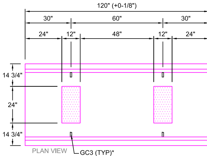
BHF4024-120 SCALE: 1/2" = 1'-0" WEIGHT: 5999#
