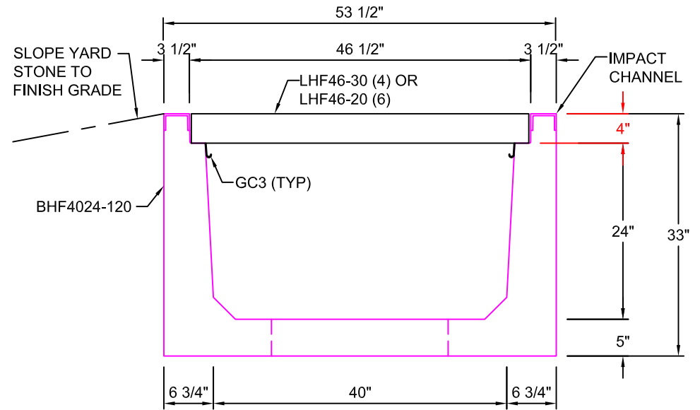
TYPICAL ROAD CROSSING SECTION WITH FIBRELITE LID 40"W x 24"D SCALE: 1"=1'-0"
