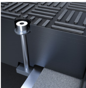
Side locking roto-latch connects to SS angle on trench wall
