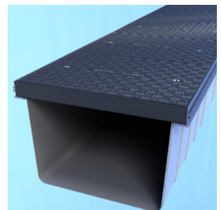
New modular GRP trench & cover
