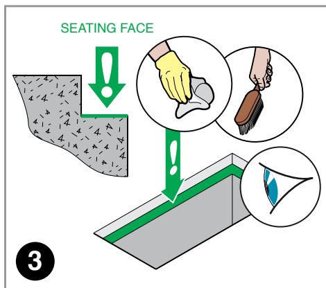
Clear and clean the frame or rebate, particularly the seating face. Inspect for damage.
