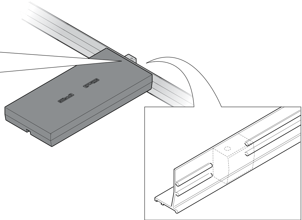
Detail showing ribs cut away to accept lock housing
